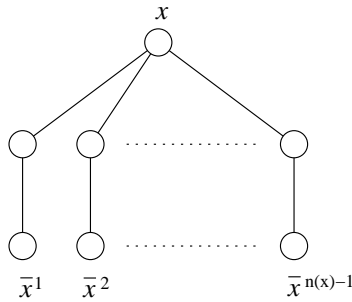
Figure 8: Subgraph T(x) .
