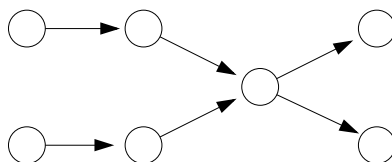
Figure 13: A graph (2, 3) -decomposable
