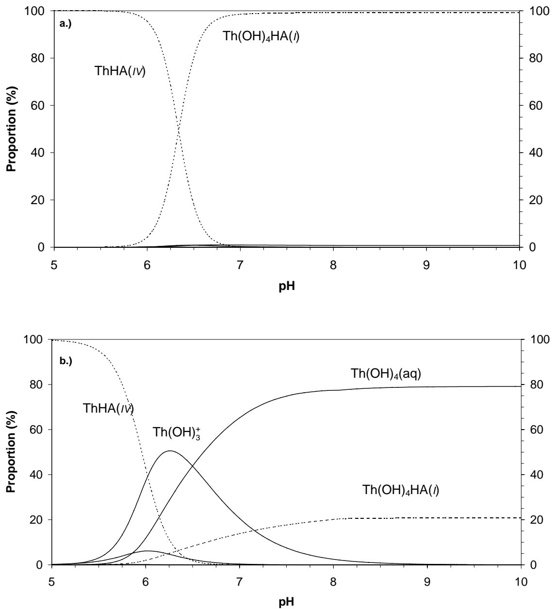
Figure 4: Speciation of thorium (IV) vs. pH taking into account \text{Th}(\text{OH})_4\text{HA}(\text{l}) with \log \beta_{1,4,1} = 41.6 referring to [61]: a. [\text{NaClO}_4] = 0.101 \text{ m} , [\text{HA}(\text{l})] = 7.8 \cdot 10^{-4} \text{ eq/L} , [\text{HA}(\text{IV})] = 1.95 \cdot 10^{-4} \text{ eq/L} ; b. [\text{NaClO}_4] = 0.101 \text{ m} , [\text{HA}(\text{l})] = 1.48 \cdot 10^{-6} \text{ eq/L} , [\text{HA}(\text{IV})] = 0.3 \cdot 10^{-6} \text{ eq/L} .
