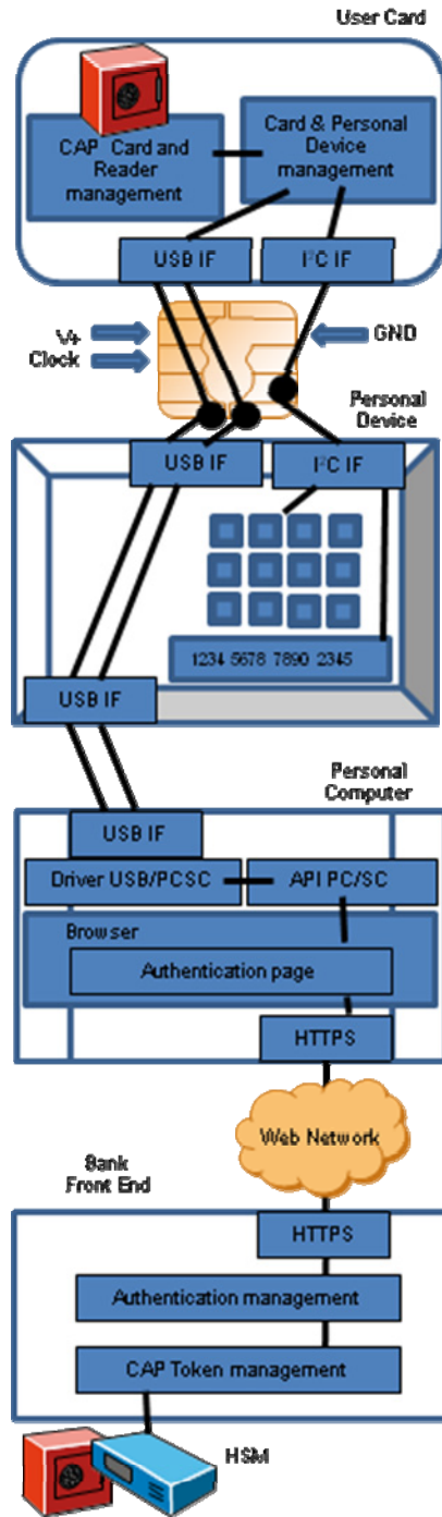
Figure 5: SOPAS architecture
