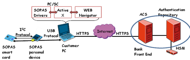
Figure 4: Interface Protocols
