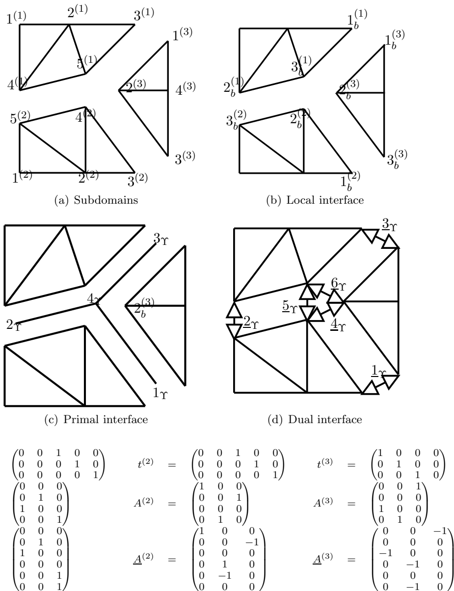
Figure 6. Local numberings, interface numberings, trace and assembly operators
