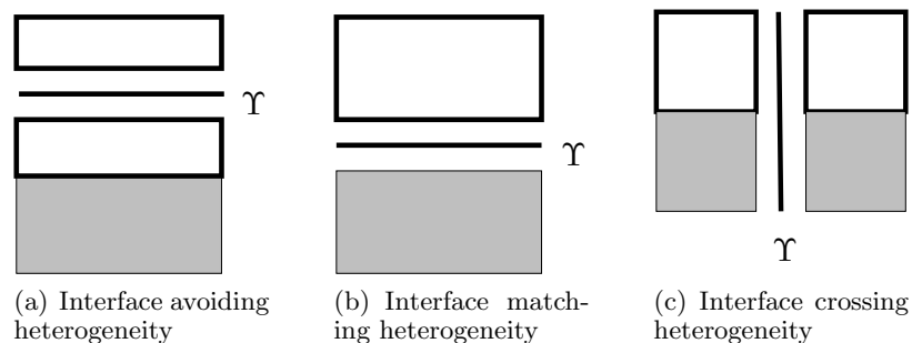
Figure 13. Different kinds of heterogeneity in domain decomposition context
