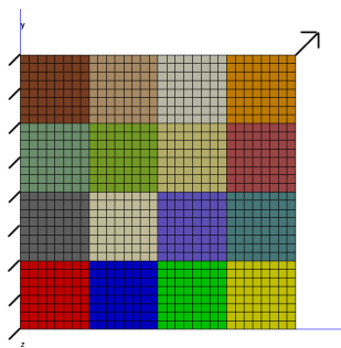
Figure 17. 16 subdomains decomposed square
