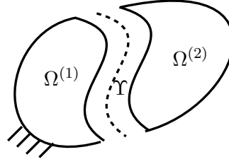
Figure 4. Two-subdomain decomposition
