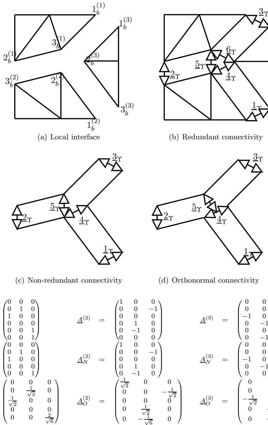
Figure 7. Suppressing redundancies of dual interface
