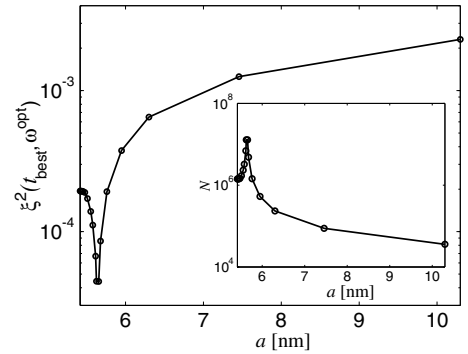
FIG. 2: Spin squeezing \xi^2(t_{\text{best}}) optimized with respect to \bar{\omega} as a function of the scattering length a , when the magnetic field is varied on the left side of the B_0 = 1007.4\text{G} Feshbach resonance of ^{87}\text{Rb} . The inset shows the number of particles for each point, calculated for \eta = 10\% . We took a(B) = a_{\text{bg}}[1 - \Delta B/(B - B_0)] with a_{\text{bg}} = 5.32\text{nm} , \Delta B = 0.21\text{G} . The three-body rate constant K_3(B) is taken from [15].
