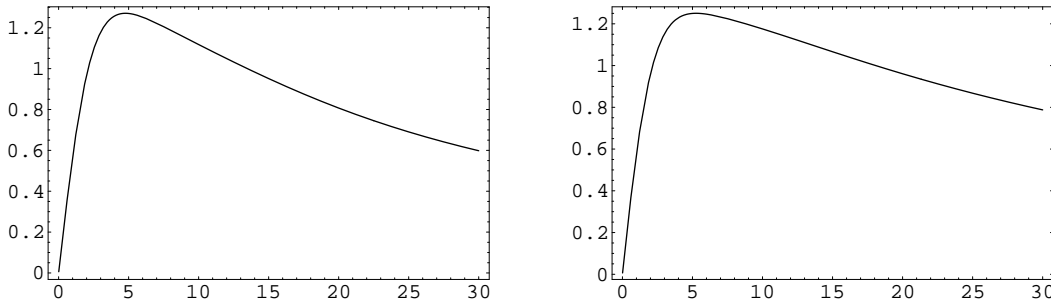
Fig. 5. Plot of the Péclet number Pe as a function of \omega in the sinusoidal case (left) and in the smooth sawtooth potential case (right).
