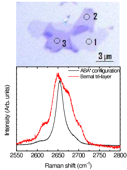
FIG. 4: (color online) Top : Optical microscope image of a thin layer (1) covered by a torn thicker layer (2). Both layers have been independently probed, (1) has been found to be graphene and (2) identified as a Bernal bilayer. The color also confirms these conclusions. The overlapping area (3) could be ABA (Bernal trilayer) or ABA' (Bernal bilayer plus a rotationally disordered graphene). Bottom : measured Raman signal on (3) (black line) compared to a reference Bernal trilayer (red line) at 633 nm. The clear difference make us state that (3) is a graphene misoriented on top of a Bernal bilayer.
