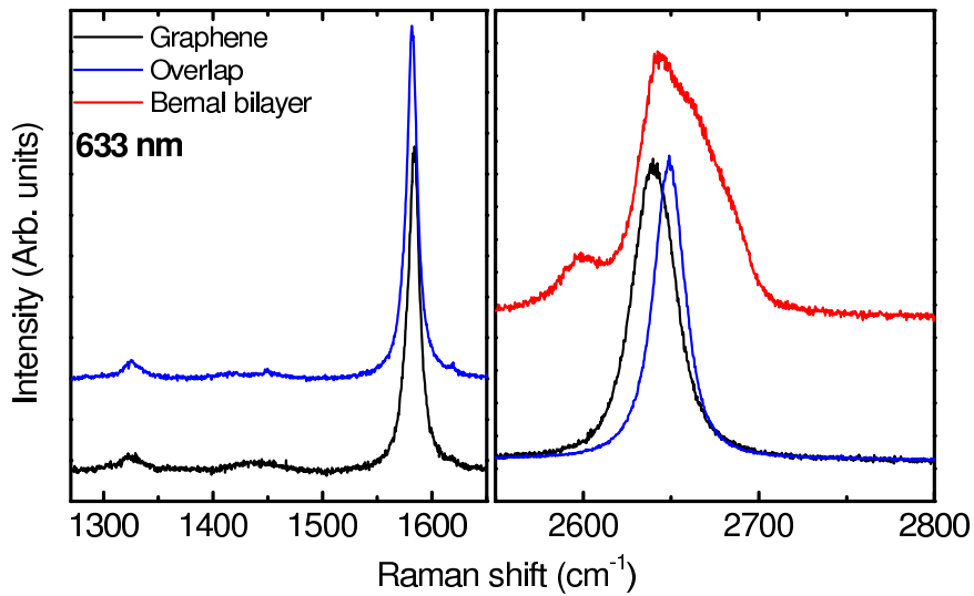
FIG. 2: (color online) Raman spectra of a single graphene sheet ( \alpha' , black lines), Bernal bilayer (red line) and two overlapping misoriented graphene sheets ( \alpha' + \alpha'' , blue lines) at 633 nm. Left : G and D band range of the graphene and overlapping configuration. Curves have been vertically offset for clarity and normalized on the G peak. The frequency shift is about 2.6 \text{ cm}^{-1} and comparable to what is reported in the literature. Right : 2D band region for single graphene sheet ( \alpha' ) and overlap ( \alpha' + \alpha'' ) compared to Bernal bilayer. The spectrum of \alpha'' is almost identical to \alpha' and will hardly be seen if plotted on the same figure. The overlapping graphene spectrum consists in a single peak clearly shifted compared to single graphene. It strongly differs from Bernal stacked bilayer (above curve). Its width ( 19 \text{ cm}^{-1} ) is smaller than the single graphene peak ( 26 \text{ cm}^{-1} ).
