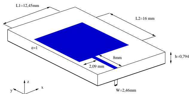
Figure 7: Patch antenna fed by a micro-strip line.
