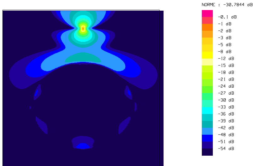
Figure 13: Electric field at frequency f = 0.5 GHz.
