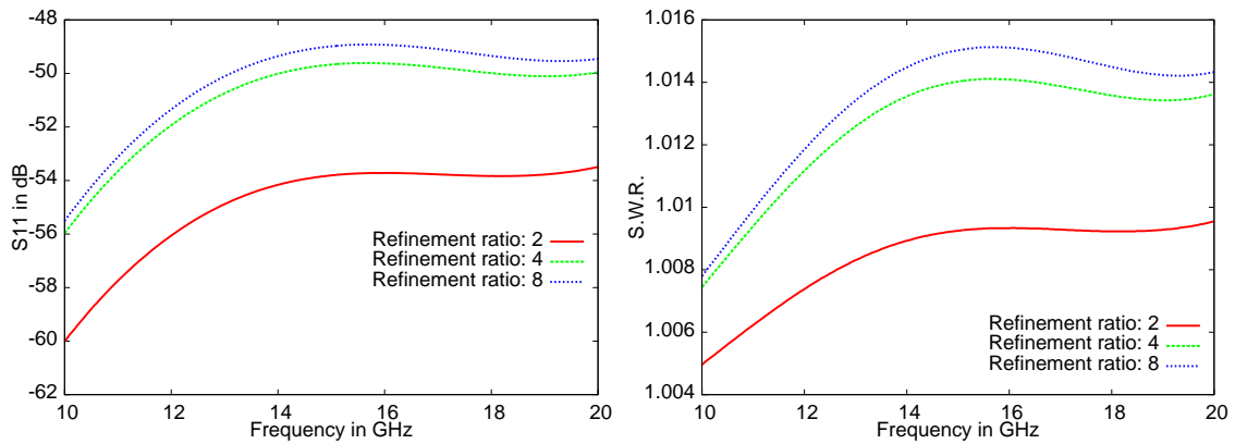
Figure 6: S_{11} and SWR coefficients for different refinement ratios k_x = k_y = k_z = 2, 4, 8
