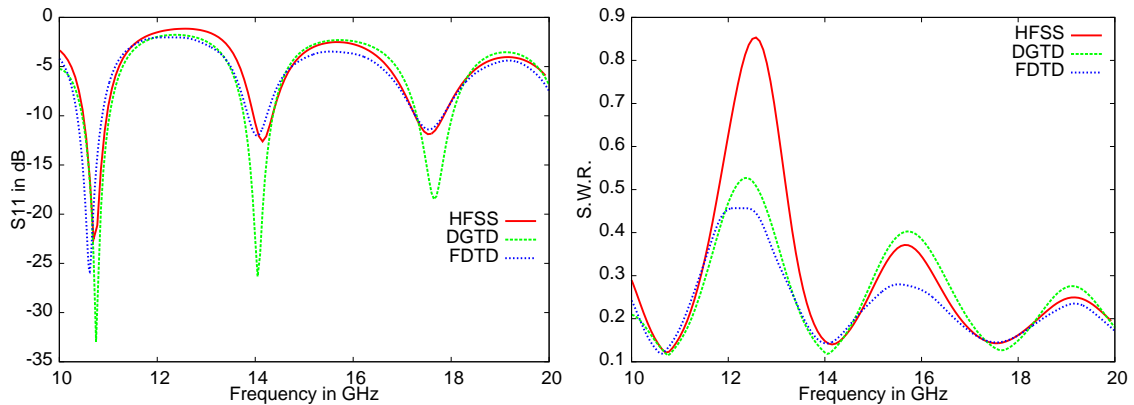
Figure 8: Values of |S_{11}(f)| (left) and SWR(f) (right) computed using: (green) DGTD- Q_{div}^1 ; (blue) FDTD; (red) HFSS.
