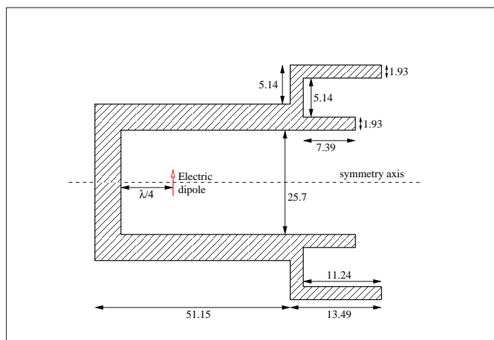
Figure 14: Cylinder horn antenna fed by an electric dipole located at \lambda_g/4 (for f = 7.5 GHz) inside the cylinder waveguide (lengths in mm ).
