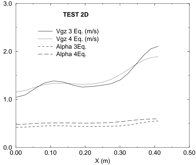
Fig. B.6. Two dimensional gas velocity profile at z=0.75\text{m}
