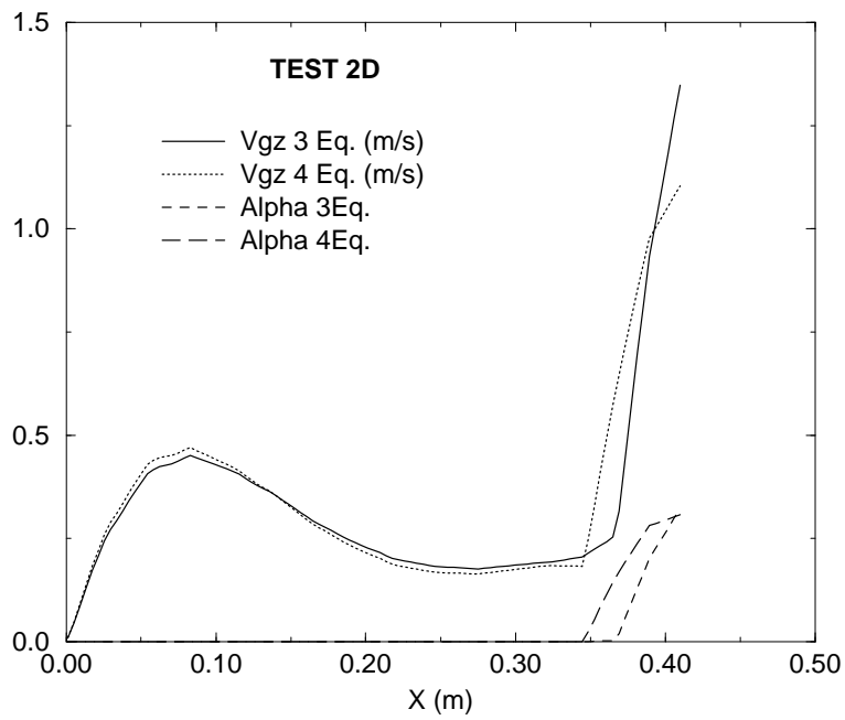
Fig. B.4. Two dimensional gas velocity profile at z=0.13 m
