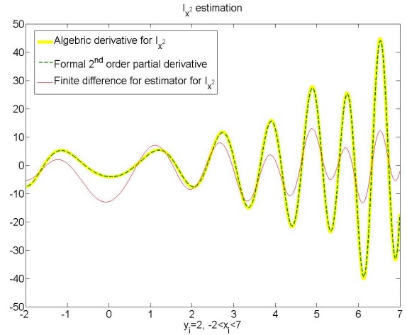
Fig. 2. Estimation of I_{x,2}
