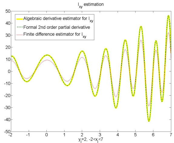
Fig. 3. Estimation of I_{xy}
