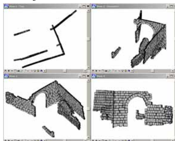
Figure 6. CAD generation of the measured blocks. (Bentley Microstation)
