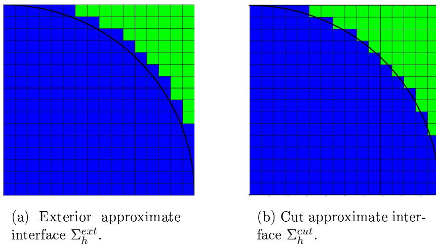
Figure 9. Non-conforming mesh, approximate interfaces \Sigma_h and approximate domains \tilde{\Omega}_h .
