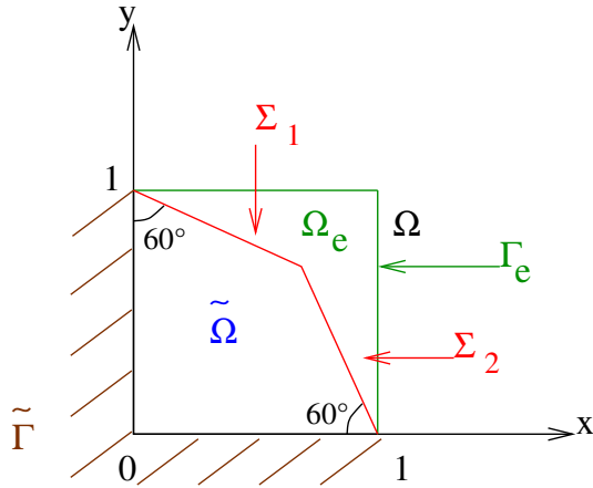
(a) Original corner domain and fictitious square domain
