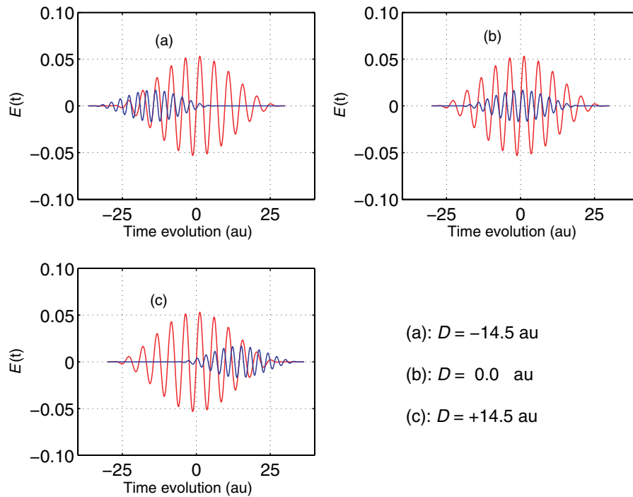
Figure 6. Electric field associated with the pulses p_1 and p_2 . Three values ((a)–(c)) of the time delay D between the two pulses are considered. The pulse characteristics are: I_1 = 10^{14} W cm ^{-2} , \omega_1 = 1.3 au, T_1 = 12 cycles, I_2 = 10^{13} W cm ^{-2} , \omega_2 = 2.1 au, and T_2 = 14 cycles. The red curve corresponds to E_1(t) and the blue one to E_2(t) .
