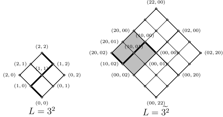
Figure 4: The lattice L = 3^2 and its bipolar extension. In bold the maximal chain corresponding to f
