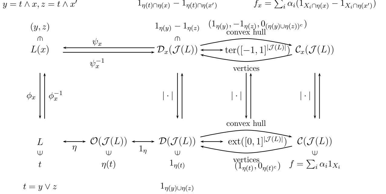
Figure 3: Relations among various concepts introduced. |\cdot| indicates absolute value, and \text{ter}() indicates vectors whose components are -1 , 1 or 0 .
