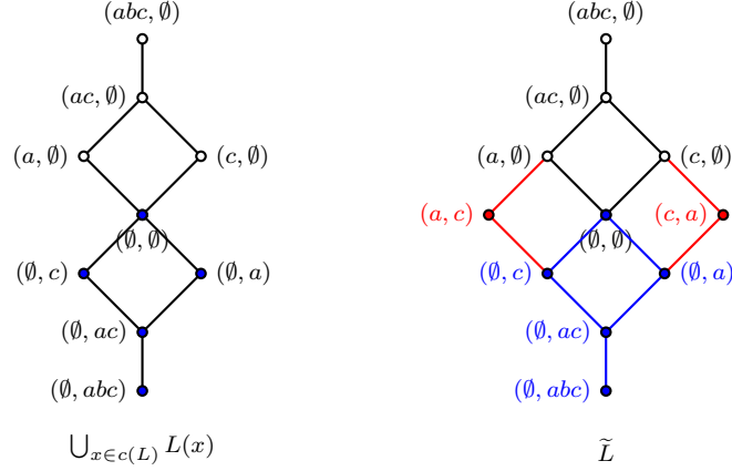
Figure 2: Left: bipolar structure computed as a replication of L . Right: the true bipolar structure
