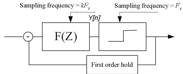
Figure 3 : Oversampled modulator.
