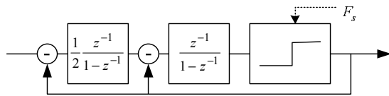
Figure 4 : DT modulator.
