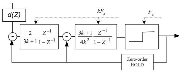
Figure 6 : Equivalent ODT modulator.
