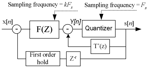
Figure 3 : ODT model with loop delay
