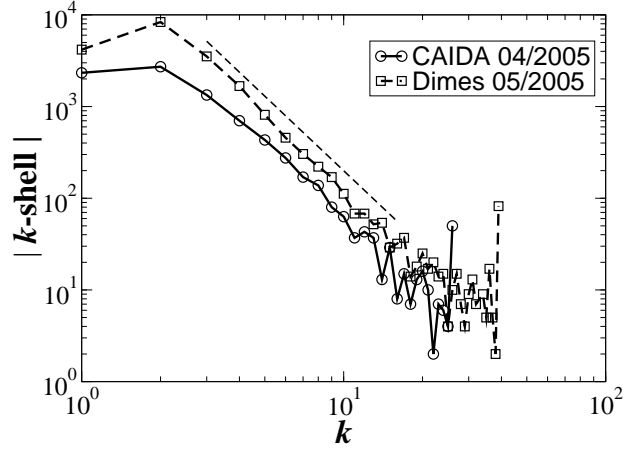
FIGURE 2. Shell size as a function of their index for the AS maps. The dashed line is a power-law \propto k^{-2.7} .
