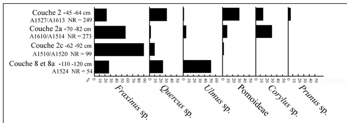
Figure 10 : Fexhe-le-Haut-Clocher "Podri l'Cortri" – Charcoal diagram of pit 61 (1)
