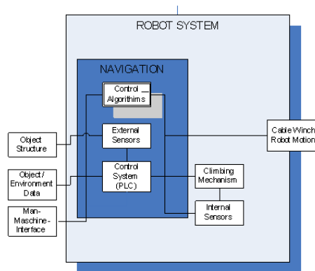
Figure 6: Control system concept
