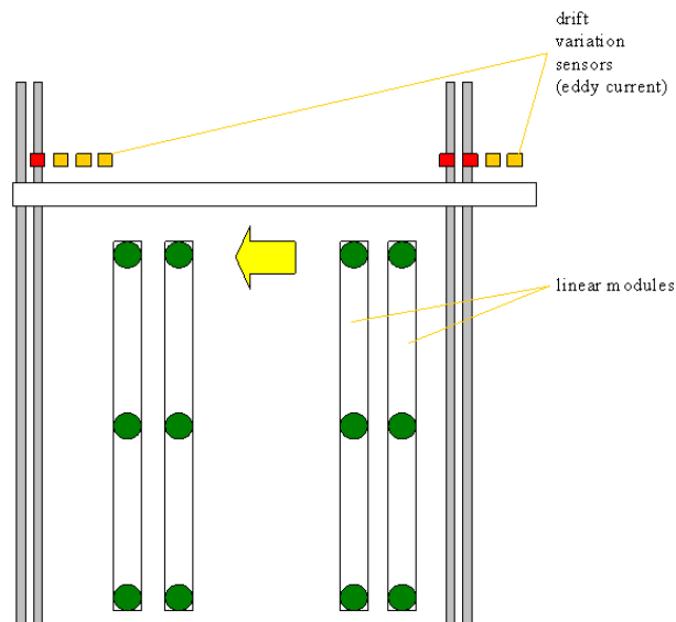
Figure 4: Schematic diagram of the detection of drift variation
