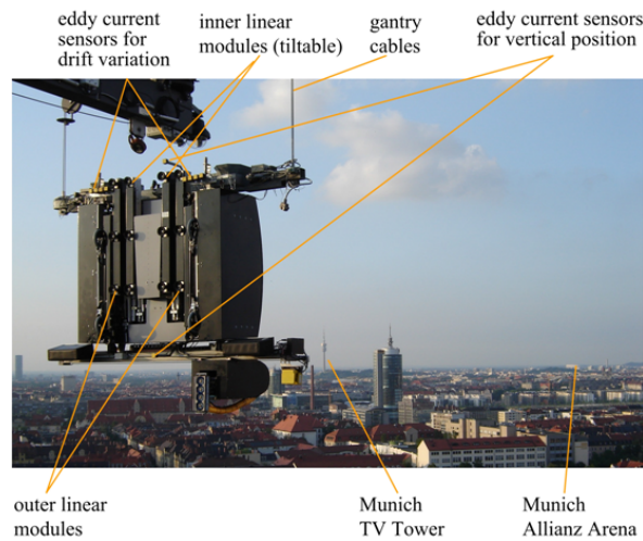
Figure 3: SIRIUSc kinematics and navigation sensors
