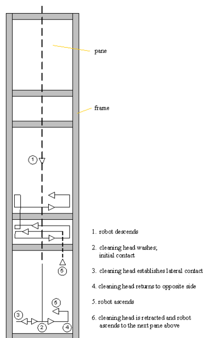
Figure 5: Robot and cleaning head motion (operation/sequence) on a pane path
