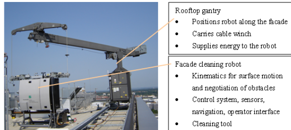
Figure 1: Rooftop gantry and facade cleaning robot atop the building
