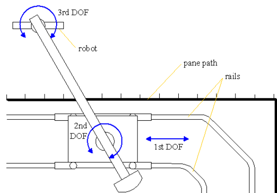
Figure 2: Gantry's degrees of freedom to position and deposit the robot on the facade
