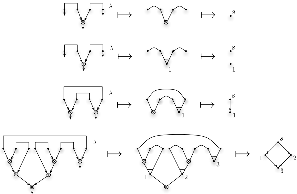
Figure 5: MLL proof structures, corresponding paired graph and dependency graphs, for the sequents A^\perp, A \otimes B, B^\perp (correct), A^\perp, A \wp B, B^\perp (incorrect), A \otimes B, A^\perp \wp B^\perp (correct) and ((A \otimes B) \wp B^\perp) \otimes (C^\perp \wp (C \otimes D)), D^\perp \wp A^\perp (correct)
