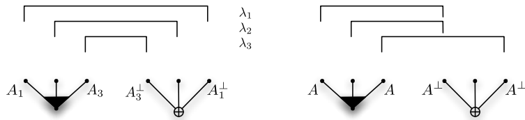
Figure 2: The MALL proof-net on \Gamma_1 , and an example of proof-net on \Gamma_2 , with n = 3 .
