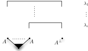
Figure 6: A proof-net (\Gamma, \Theta) , with \Theta = \bigcup_{i=1}^n \lambda_i .
