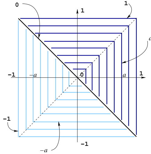
Figure 1: Constant level curves of the symmetric maximum
