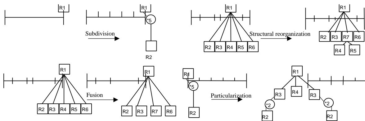
Figure 5: Schema of some operations on the rules
