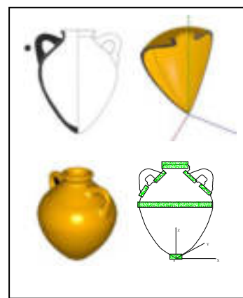
Fig.5. Ideal amphora model: from archaeologist design to digital model
