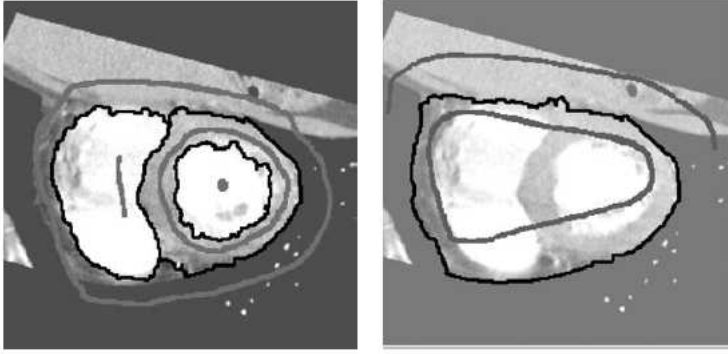
FIGURE 4.1. (Taken from [19].) The Grady segmentation method is a linearized sigma filter applied to propagate seed regions. The grey curves are user defined seed region. In that case one of the seed region is put to 1 and the other to zero. A diffusion with sigma filter weights computed on the original image u_0 is applied until a steady state is attained. This gives at each pixel \mathbf{y} a value p_1(\mathbf{y}) between 0 and 1 which is interpreted as the probability for \mathbf{y} to belong to the region of the first seed. A threshold at 0.5 gives the black curves separating the regions of both seeds. Like the active contour method, this method is highly dependent on the initial seeds. It is, however, much less sensitive to noise than the snakes method and permits to initialize fairly far from the desired contours. We shall see that by the histogram concentration effect one can get similar or better results without any initialization. See Section 4.1.
