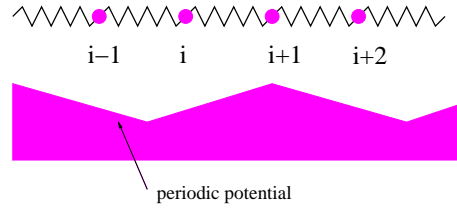
Figure 1: Sketch of the chain or particles for the classical FK model
