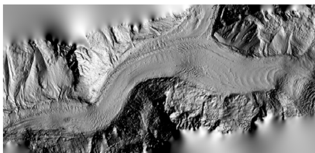
Figure 3. Mer-de-Glace and Tacul glaciers, high resolution DTM from airborne photographs, August 95.
