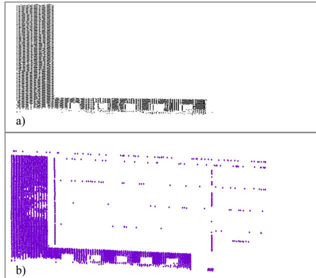
Figure 9. Representation of a planar wall, extracted in two ways; a) manual extraction; b) automatic extraction.
