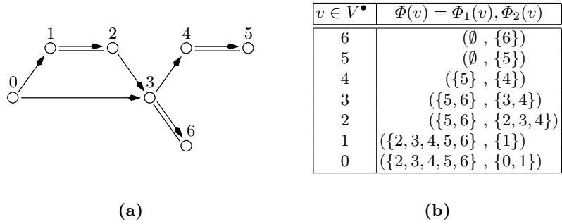
Fig. 6. (a) A mixed graph G^* = (V^*, A^*, E^*) , labelled in topological order, and (b) the edges to propagate with respect to the order described by arcs, for each node v in \Phi_1(v)
