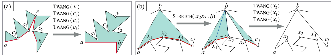
Figure 8: Reverse atomic moves: (a) \text{STRETCH}(ab, v) is reversed by \text{TWANG}(v) , \text{TWANG}(c_1) , \text{TWANG}(c_2) , \text{TWANG}(c_3) . (b) \text{TWANG}(b) is reversed by \text{STRETCH}(x_2x_3, b) , \text{TWANG}(x_2) , \text{TWANG}(x_1) and \text{TWANG}(x_3) .
