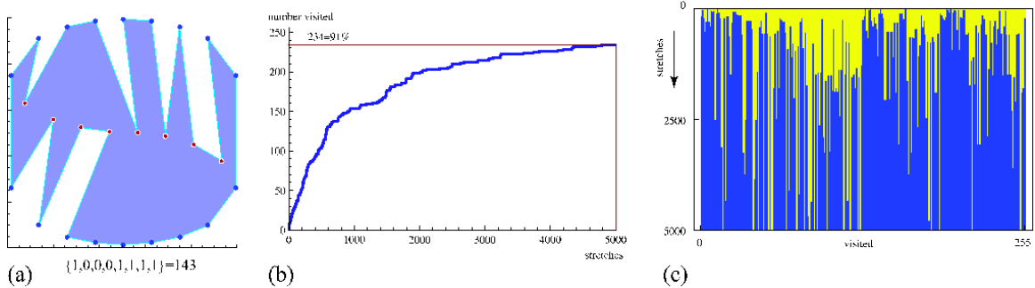
Figure 9: k=8 , 2^k=256 . (a) Polygonization \rightarrow bits map. (b) Numbers visited vs. stretches. (c) Dark: numbers visited with increasing stretches; light: not yet visited.
