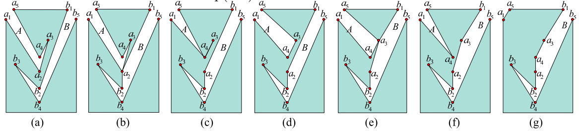
Figure 6: SINGLE POCKET REDUCTION( P, a_1a_5 ) illustrated: (a) Initial P ; (b) After \text{STRETCH}(b_1b_2, a_2) ; (c) After \text{TWANG}(a_1a_2a_3) ; (d) After \text{TWANG}(a_3a_4a_5) ; (e) After \text{STRETCH}(a_2b_1, a_3) ; (f) After \text{TWANG}(a_4a_3a_5) ; (g) After \text{STRETCH}(a_2a_3, a_4) + \text{TWANG}(a_1a_4a_5) .
