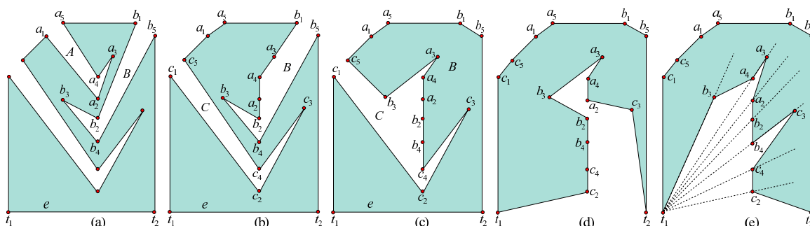
Figure 7: (a-e) POCKET REDUCTION( P, t_1t_2 ): (a) Initial P ; (b) After SINGLE POCKET REDUCTION( P, a_1a_5 ); (c) After SINGLE POCKET REDUCTION( P, b_1b_5 ); (d) After SINGLE POCKET REDUCTION( P, c_1c_5 ); (e) After CANONICAL POLYGONIZATION( P, t_1t_2 ).
