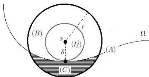
FIGURE 1. Domain decomposition
