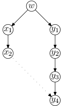
Figure 1: \hat{\varphi}^{2 \rightarrow 4}
