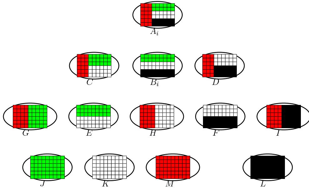
Figure 3: Cantor-Bendixson ranks
