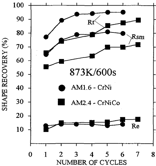
Figure 3. Shape recovery as a function of training cycle for CrNi alloy and CrNiCo alloy annealed at 873K.
