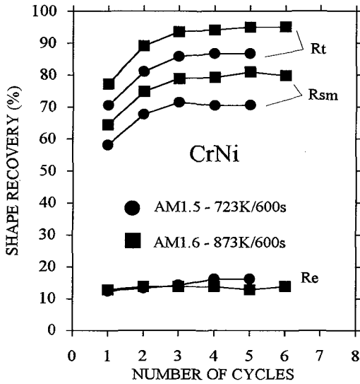
Figure 1. Shape recovery as a function of training cycle for CrNi alloy annealed at 723K and 873K respectively.
