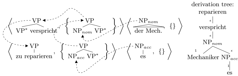
Fig. 3. TT-MCTAG derivation of (1)
