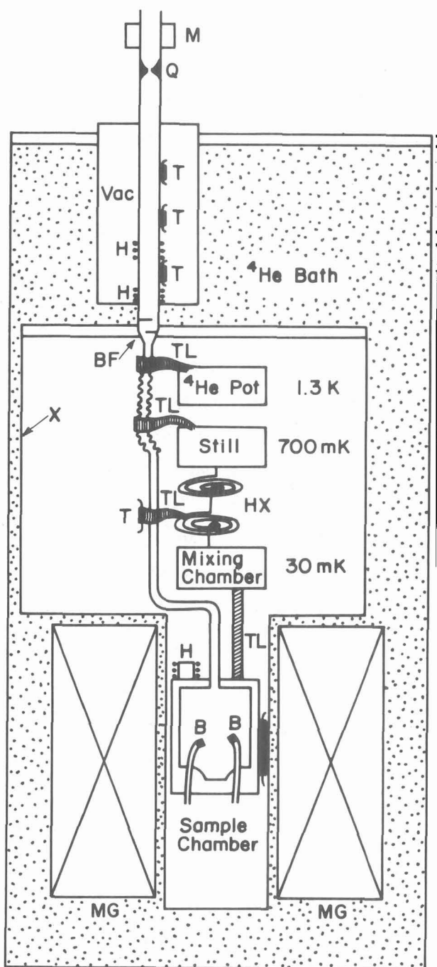
FIGURE 1. Cryostat for production of spin polarized hydrogen (not drawn to scale). M is the 2.45 GHz microwave cavity, Q is the .77 mm diameter quartz orifice, Vac is the vacuum jacket, T corresponds to the thermometer, H corresponds to the heater, BF is the radiation and thermalization baffle, TL corresponds to the thermal link, X is the exchange gas can, HX is a continuous counter-current exchanger, B is the bolometer and MG is the 60 kG magnet. 30 mK is the lowest mixing chamber temperature attained. With a 60 kG magnetic field, a ^4\text{He} film in the sample chamber and hydrogen flowing into the cryostat, the temperature of the mixing chamber is considerably higher.
