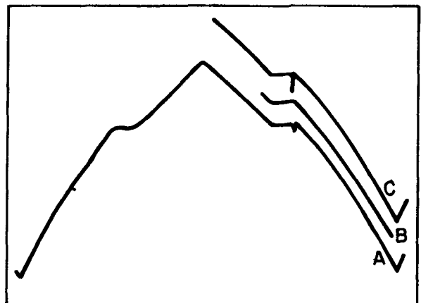
FIGURE 2. Bolometer voltage response for a sawtooth variation of bolometer current. Time starts on the right hand side of the figure. The current increases until a plateau is reached corresponding to boiling the ^4\text{He} film away from the bolometer. Trace A shows the bolometer response with a 60 kG field on after 10 minutes of H atom accumulation. The small downspike at the break in slope of trace A corresponds to heating by recombination of H atoms. Trace B gives the bolometer response after 10 minutes of H atom flow with zero magnetic field. No downspike is observed. Trace C shows the bolometer response curve taken after the field was ramped up from 0 to 60 kG in a period of 15 minutes followed by a 10 minute period at 60 kG. A larger recombination feature can be observed.
