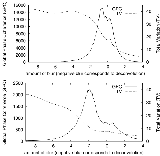
Fig. 4. Top: Graphs of r \mapsto GPC(h_r \star u) and r \mapsto TV(h_r \star u) , where u is the Lacornou image and h_r is a deconvolution kernel ( r < 0 ) or a blur kernel ( r > 0 ) (see Equation 2). Bottom: same experiment applied to u' = g_2 \star u + w , where w is a Gaussian white noise with unit variance. Contrary to a simple TV measurement, the GPC permits to select the best deconvolution parameter r as the one producing the image with the most coherent phases. The original Lacornou image can be slightly improved (GPC is maximum for r = -0.6 ), and the parameter of the blur kernel used to produce the degrade version is well recovered (GPC is maximum for r = -2.1 ).
