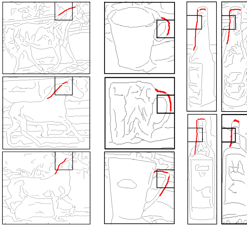
Fig. 5. One of the most important window descriptor dimensions, according to SVM training ( k = 2 ). Each column shows a few training images for a class, along with one of the ‘ k AS type + tile’ combinations which are given the highest weight by the SVM.
