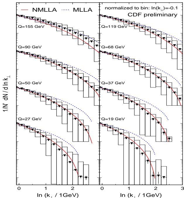
FIG. 4: CDF preliminary results for the inclusive k_{\perp} distribution at various hardness Q in comparison to MLLA and NMLLA predictions at the limiting spectrum; the boxes are the systematic errors (their lower limits at large k_{\perp} are cut for the sake of clarity).
