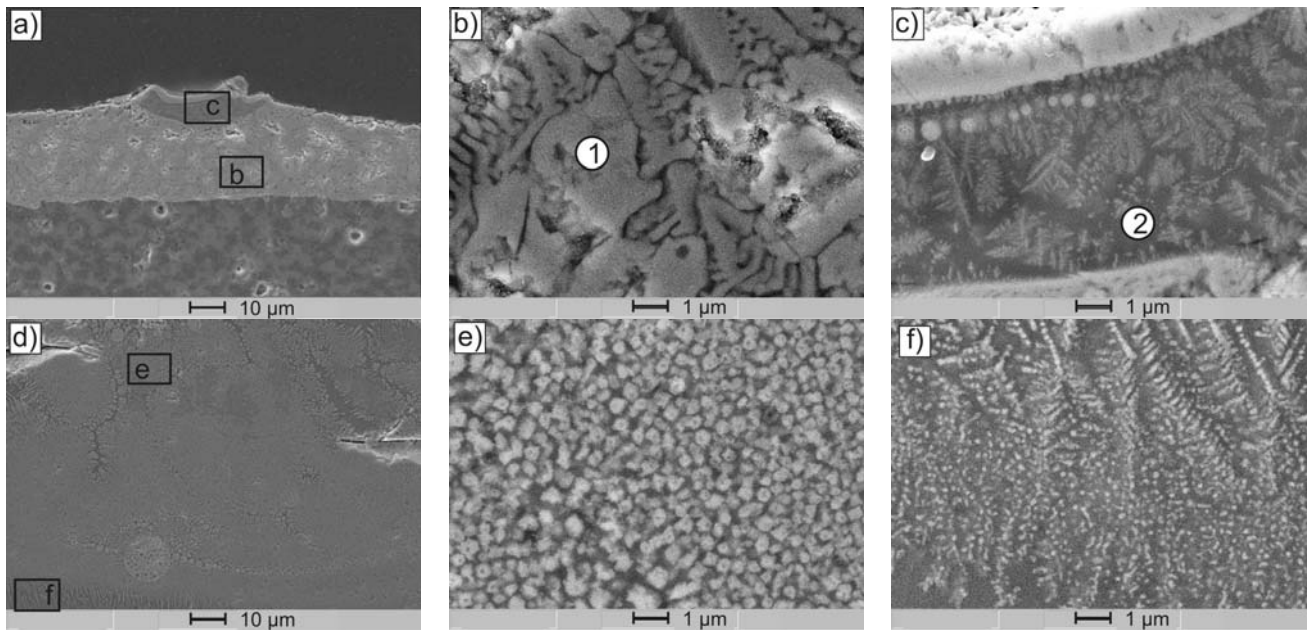
Fig.4.: SEM-images of laser alloyed LTCC with nano-CuO; a),b),c) of a layer located at the top of the ceramic surface and d),e),f) of a developed melt pool.
