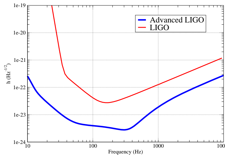
Figure 4. Advanced LIGO sensitivity vs LIGO one.
