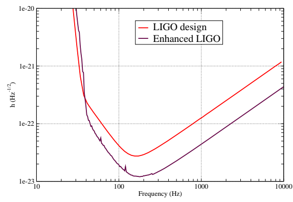
Figure 2. Enhanced LIGO sensitivity.
