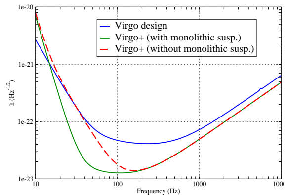
Figure 3. Virgo+ sensitivity.
