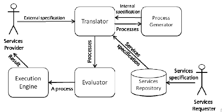
Fig. 1 The framework of the service composition system
