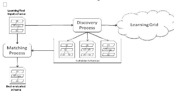
Fig. 1 Grid Learning Services automatic composition
