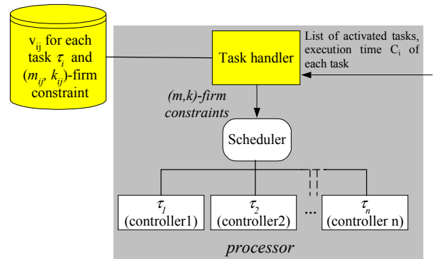
Figure 2. scheduling architecture
