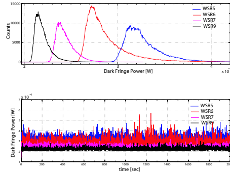
Figure 3: Dark Fringe power histogram (upper plot) and in time domain (lower plot) for the different Weekly Science Runs ; we can notice a progressive improvement in stability and darkness of the dark port signal mainly due to the continuous improvement in the filtering path of the automatic alignment control chain.
