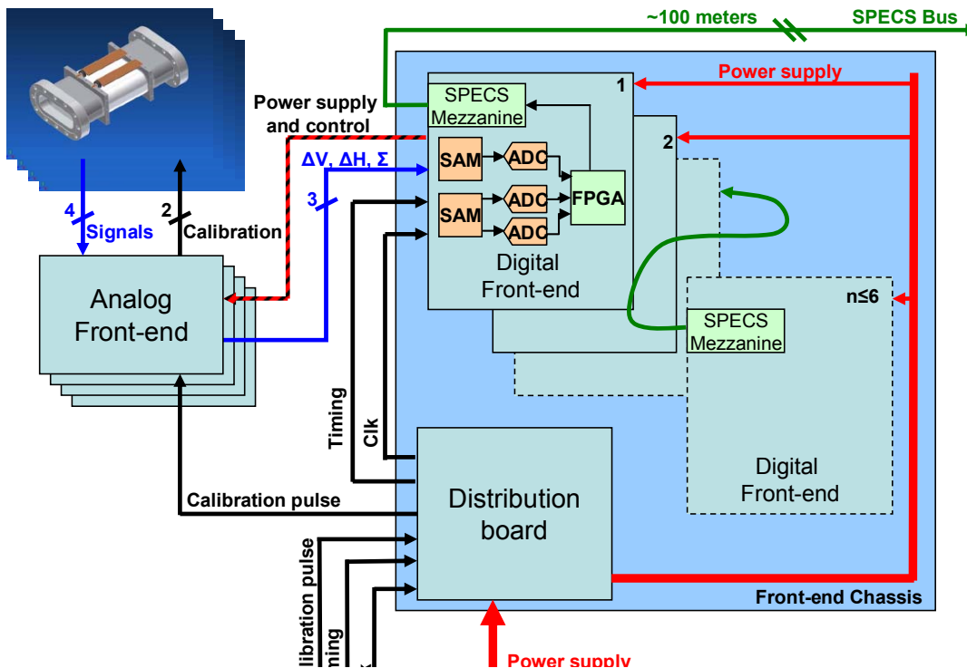
Figure 2 Hardware configuration
