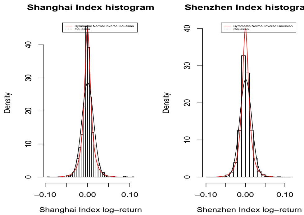
Fig. 3. Symmetric NIG fitting for log-returns of Shanghai Stock Composite Index and Shenzhen Stock Composite Index
