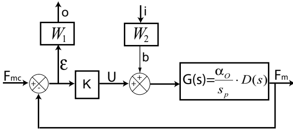
Fig. 13. The closed-loop scheme with the weighting functions.
