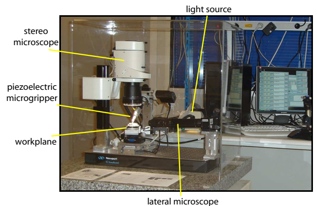
Fig. 1. Photography of the microassembly system used at the LAB. The piezoelectric microgripper is moved by a linear-angular axis. The workplane enables X - Y - \theta motions, a stereomicroscope equipped with a deported light offers a view from the top and a PC is used to control all these devices together.
