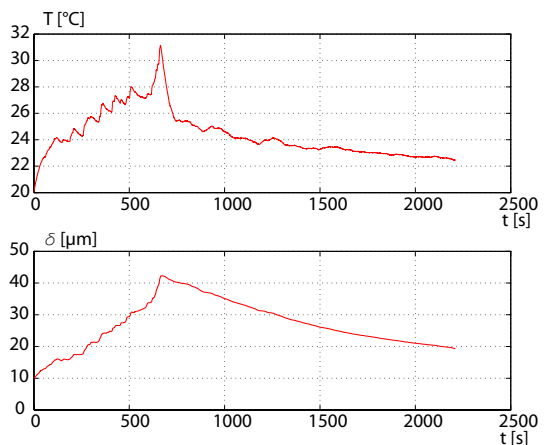
Fig. 4. Evolution of the deflection when the temperature varies (with U = 15\text{V} ).
