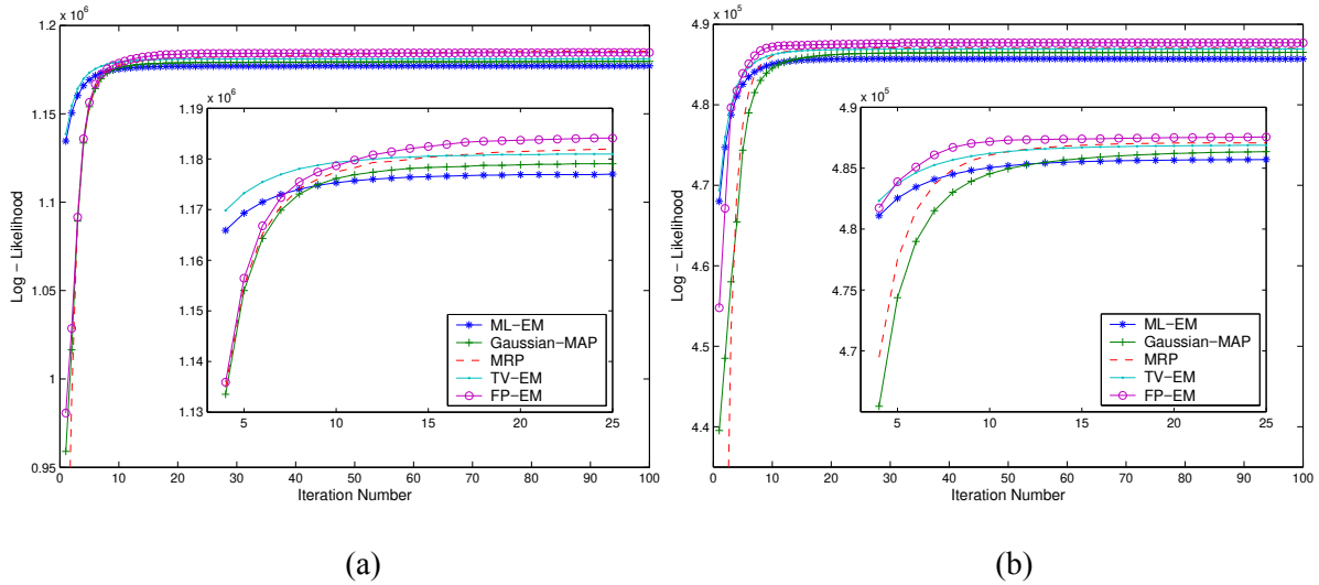
Fig. 5 Comparison of log-likelihood function increase rates of ML-EM, Gaussian-MAP, MRP, TV-EM, and FP-EM algorithms. (a) Noiseless Projections (b) Projections including 6% uniform Poisson distributed background events.
