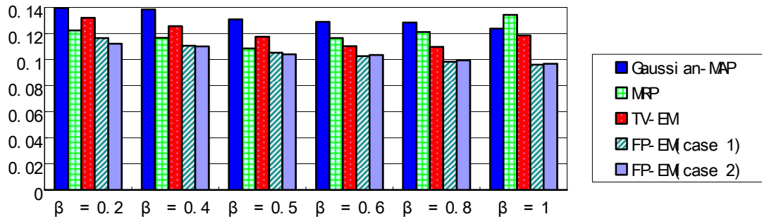
Fig. 9 The MSE of Shepp-Logan phantom including 6% uniform Poisson distributed background events obtained by running 100 iterations for the Gaussian-MAP, MRP, TV-EM, and FP-EM algorithm using different regularization parameter \beta . Case 1: Triangle member function was used for FP-EM. Case 2: Trapezium membership function was used for FP-EM
