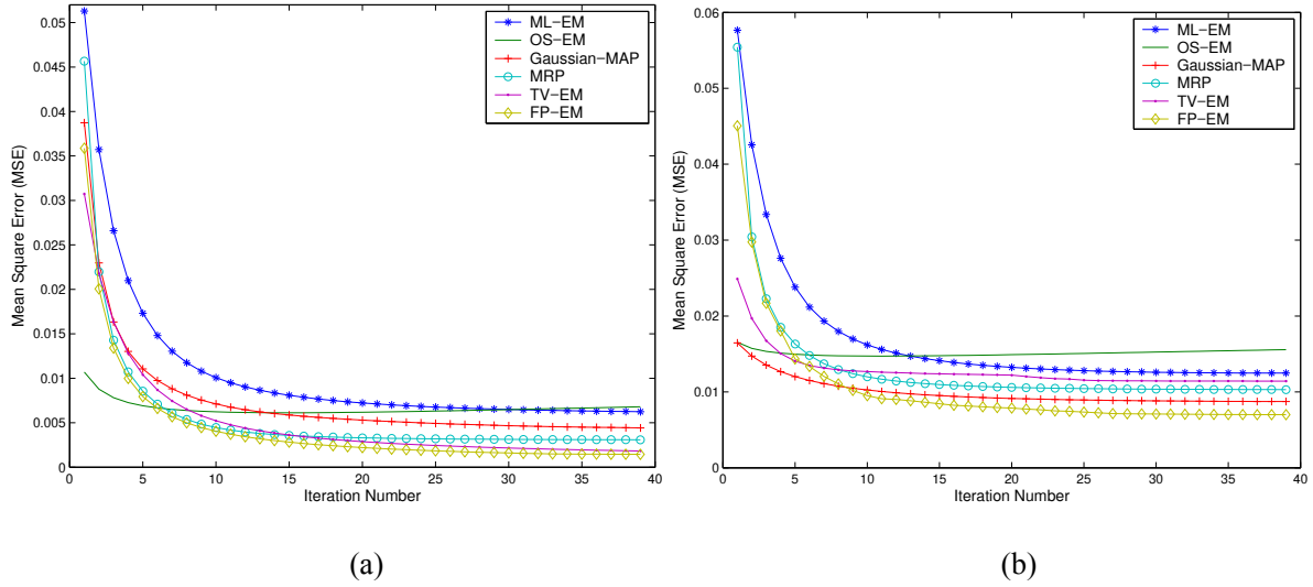
Fig. 11 MSE versus iterations. (a) Projection contained Poisson noise. (b) Projection contained by zero mean value Gaussian noise with variance 0.005
