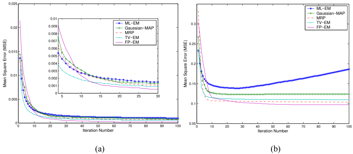
Fig. 6 Comparative analysis of MSE versus iteration number. The MSE for the ML-EM, Gaussian-MAP, MRP, TV-EM, and FP-EM algorithms (a) Noiseless Projections (b) Projections including 6% uniform Poisson
