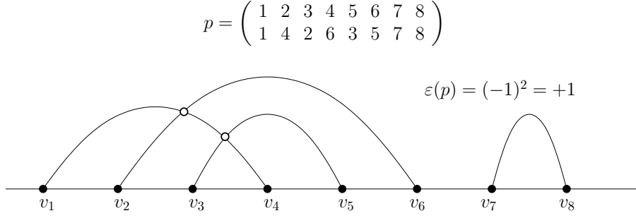
Figure 1: Diagrammatic representation of a pairing p
