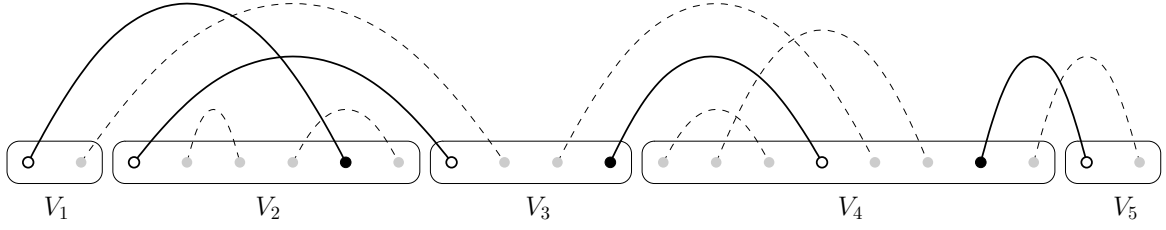
Figure 3: The exit graph \text{ex}(p) (solid lines) for p \in \mathcal{P}(\Pi)
