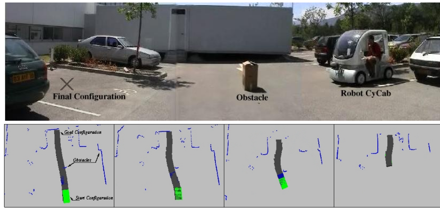
Fig. 8. A trajectory planned by robot CyCab from a parking lot to another. On top, experiment situation. On bottom, the trajectory deformation, bird's-eye viewed. An obstacle lies on the trajectory, and the CyCab has to deform its trajectory at execution time.
