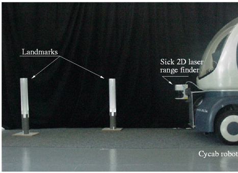
Fig. 7. CyCab robot and landmarks
