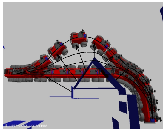
Fig. 2. Direction of deformation created by unexpected obstacles
