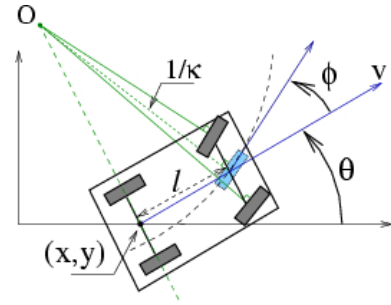
Fig. 3. Car Kinematic Model. Four configuration variables x, y, \theta, \phi . Curvature \kappa is derived from steering angle \phi and distance l to rear axle.
