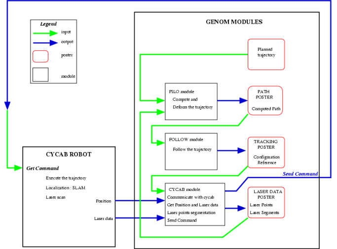
Fig. 6. Software Architecture of the Non-Holonomic path Deformation Method Integration on Robot CyCab. The CyCab communicates with GenoM modules: the two systems are distinct.
