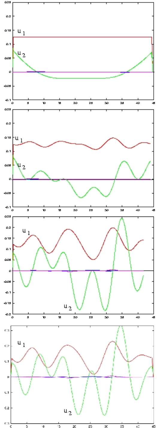
Fig. 9. Input perturbations : effect of the deformation on inputs u_i(s) along the trajectory ( s \in [0, 45] ). At the top, the inputs computed for the planned path, and below the input computed by the deformation. As the deformation process goes along, u_1 and u_2 are more and more perturbed, in order to avoid the obstacles.
