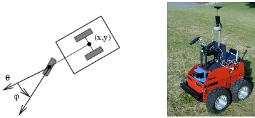
Fig. 5. Mobile robot Dala as a car-like robot: a non-holonomic system of dimension 4 with two non holonomic constraints.
