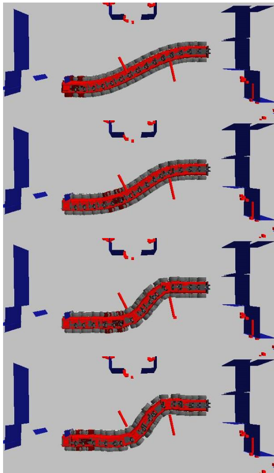
Fig. 10. Trajectory deformation. Two obstacles detected by a laser range finder lie on the path planned by the robot Dala (at the top). The trajectory is deformed in order to get a collision free path (at the bottom).
