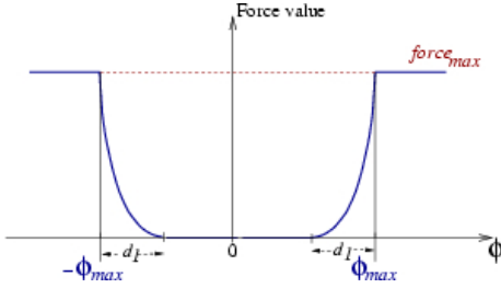
Fig. 4. Norm of the “force” \mathbf{f}_\phi(\mathbf{q}) due to the steering angle. The gradient of the potential field is indeed equivalent to a force. The value of the norm of the “force” increases when the steering angle gets closer to its bound.
